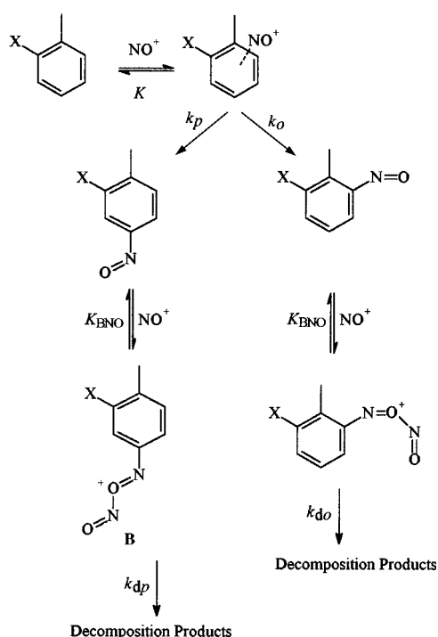
Scheme 4 For toluene ( X = \text{H} ) and o -xylene ( X = \text{Me} ).
