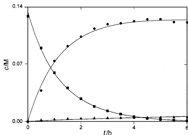
Fig. 2 Concentrations of m -xylene (■), 1,3-dimethyl-4-nitrosobenzene (●) and 1,3-dimethyl-4-nitrobenzene (▲) in the nitrosation of m -xylene in anhydrous trifluoroacetic acid under NO at 28 °C. [\text{NO}^+] = 0.450 \text{ mol dm}^{-3} .
