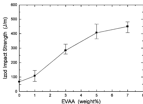
Figure 3 Compatibilizing effect of EVAA on notched impact strength of nylon 6/EVA blends.
