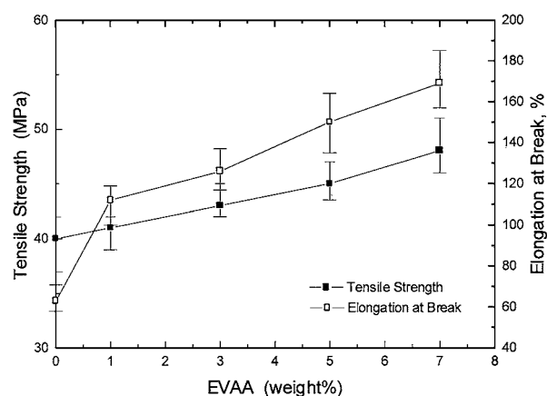
Figure 2 Compatibilizing effect of EVAA on tensile strength and elongation at break of nylon 6/EVA blends.
